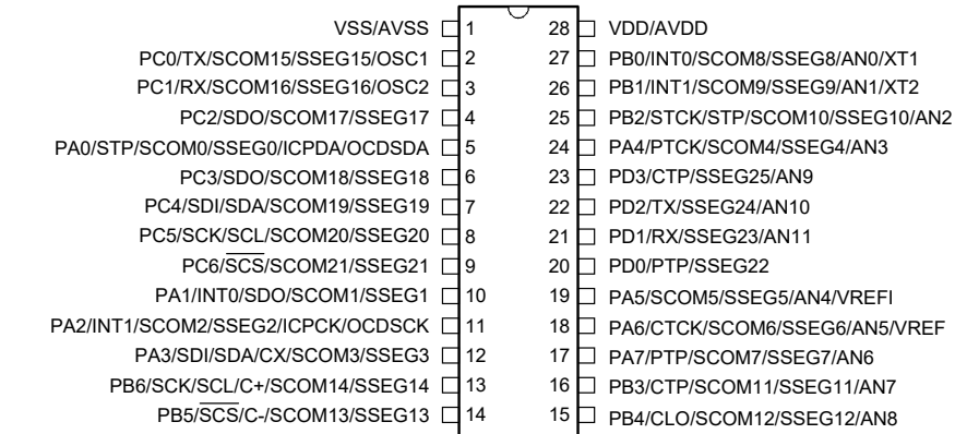
HT66F3195/HT66V3195 28 SSOP-A
