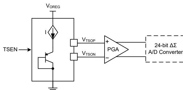
Temperature Sensor Structure
