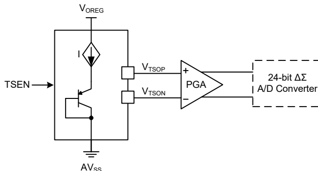
Temperature Sensor Structure
