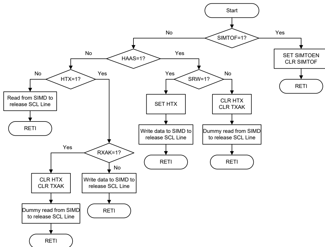
I²C Bus ISR Flow Chart
