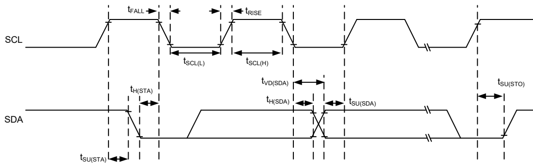
I 2 C Timing Diagram
