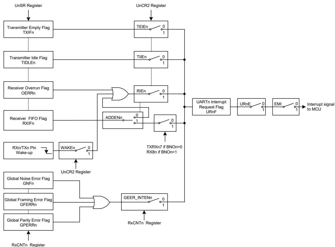
UARTn Interrupt Structure (n=0~1)
