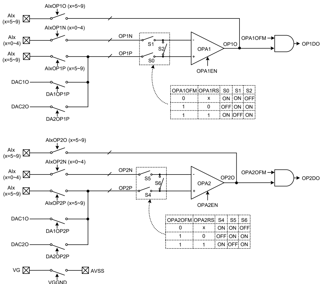
Operational Amplifier Structure
