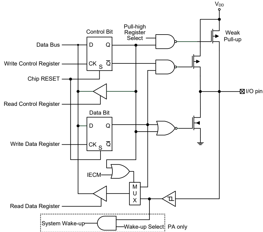
Logic Function Input/Output Structure
