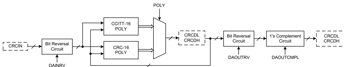
CRC Block Diagram
