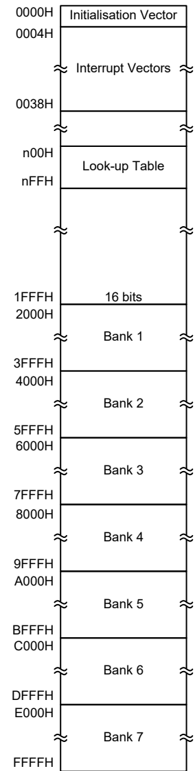
Program Memory Structure
