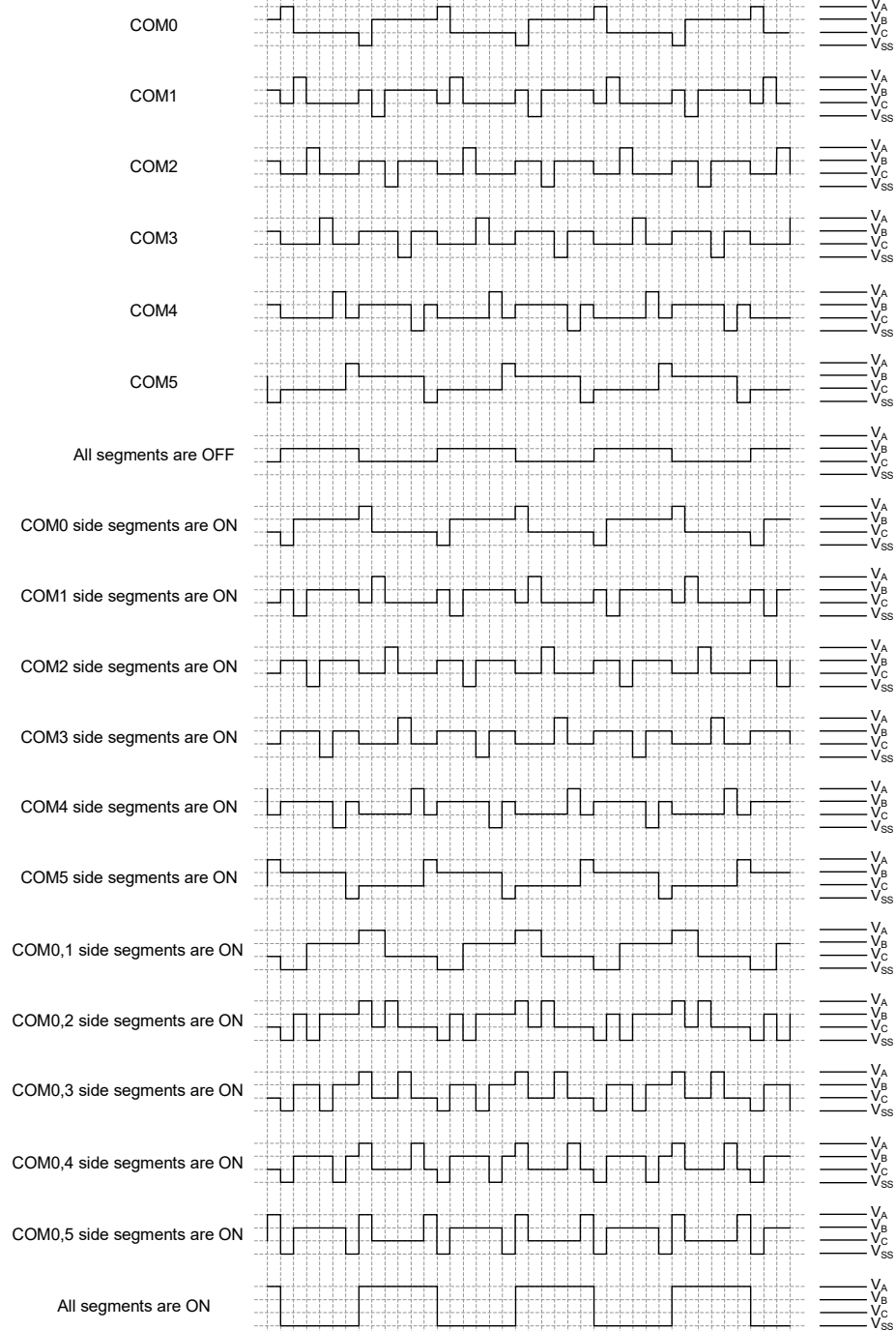
LCD Driver Output – Type B, 1/6 Duty, 1/3 Bias
