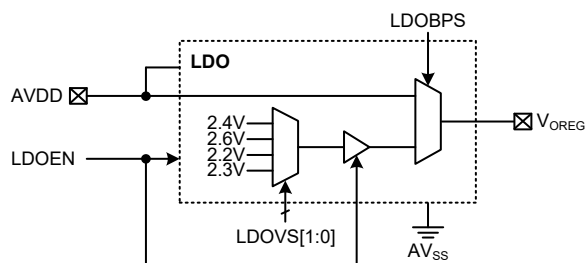
Internal Power Supply Block Diagram
