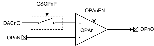
Operational Amplifier Structure (n=1~3)
