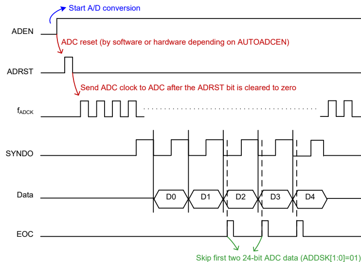
A/D Converter CTRL Unit Timing Chart – ADDSK[1:0]=01
